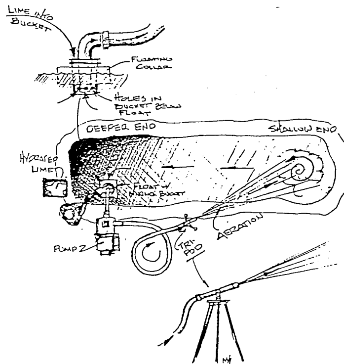
Figure III-2: Pit Treatment/Circulation
